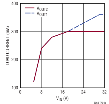
Maximum Load Current vs V_{IN}
