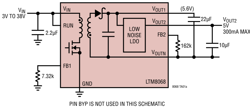
2kVAC Isolated Low Noise μModule Regulator
